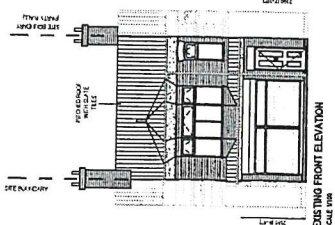
EXISTING FRONT ELEVATION SCALE 1:100
