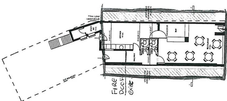
PROPOSED GROUND FLOOR PLAN SCALE 1:100
